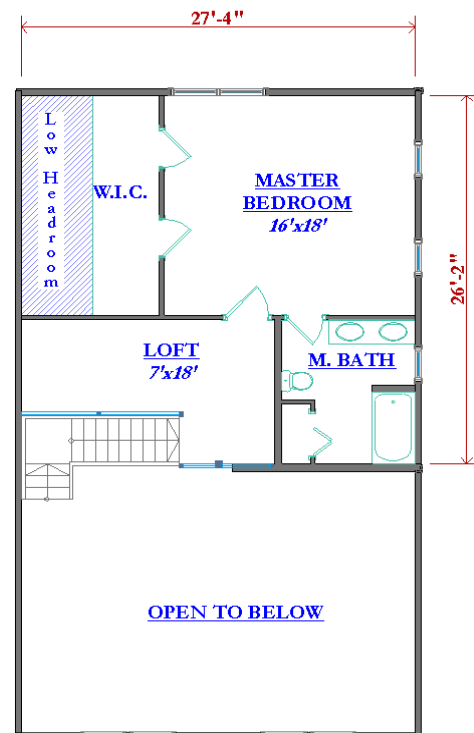
KENNEBEC 2nd Floor
